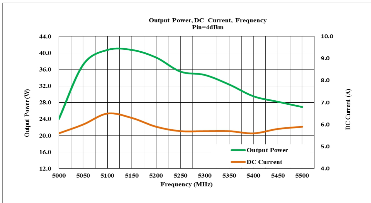
Graph 3: Output Power (Normal temp. +25\pm 3^{\circ}\text{C} )
