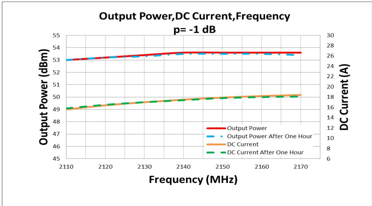
Graph2: Output Power (High temp. +60\pm 3^{\circ}\text{C} )
