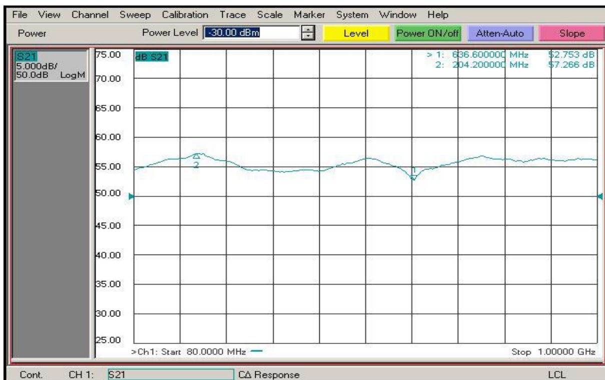
Graph4: Power Gain
