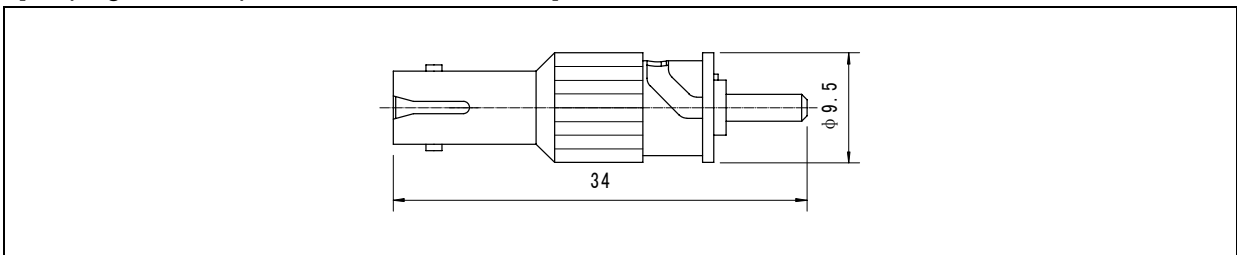
[LC plug and receptacle attenuator: AT-LC]
