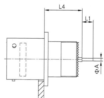
receptacle (RF27656)
