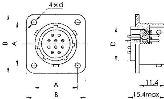
Receptacle without tail attached (pin)
