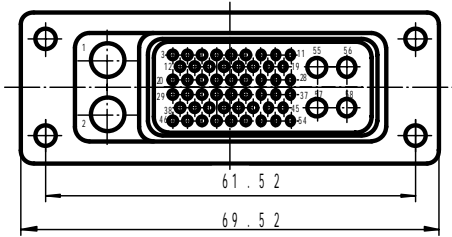
52 - \Phi 0.8 , 4 - \Phi 1.5 , 2 - Coaxial
