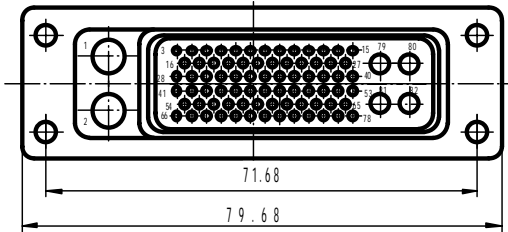
76 - \Phi 0.8 , 4 - \Phi 1.5 , 2 - Coaxial
