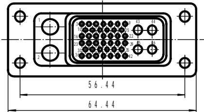
40 - \Phi 0.8 , 4 - \Phi 1.5 , 2 - Coaxial
